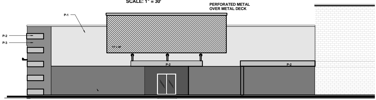
SOUTH ELEVATION SCALE: 1" = 30'
